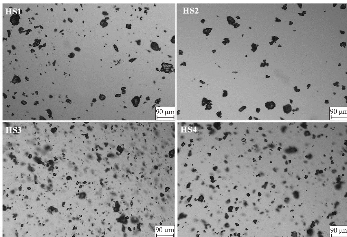
Fig. 1. Microscopic images of hydrogels containing sulfur (HS1–HS4) under magnification 100×
