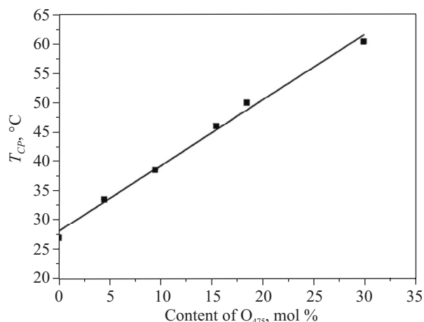
Fig. 6. Cloud point temperature T_{CP} of the copolymers P[(TEGMA-EE)- co -(OEGMA-ME 475 )] as function of the content of OEGMA-ME 475 ; reprinted with permission from Trzebicka B., Szweda D., Rangelov S. et al. : Journal of Polymer Science Part A: Polymer Chemistry 2013, 51, 614, copyright (2013) Wiley-VCH GmbH & Co. KGaA, Weinheim [39]
