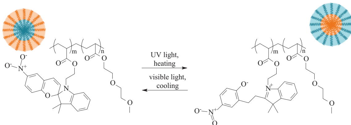
Fig. 8. Self-organization of the block copolymer PSPMA- b -P(DEGMA-ME) to micelles in water solution under the influence of light and temperature stimulus
