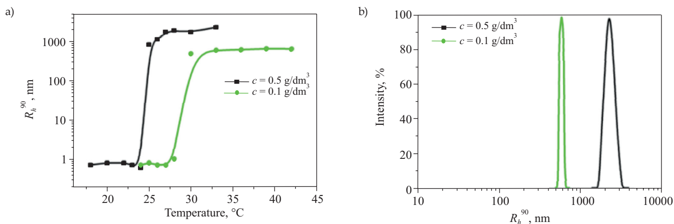
Fig. 4. Aggregation of OEGMAs: a) apparent hydrodynamic radius ( R_h^{90} ) as function of temperature for water solutions of P(TEGMA-EE), b) size distribution of formed mesoglobules
